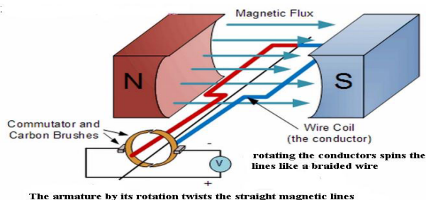
Figure 9: Electrical Generator
