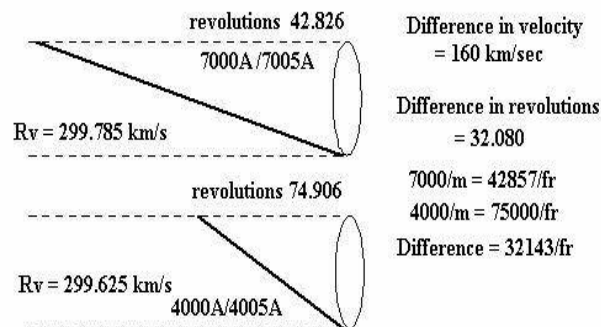
Figure 6: Statistics
