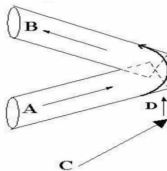
Figure 12: Light Reflection
