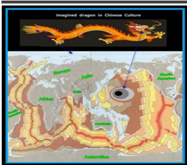
Figure 1: The "ω" Shape Giant Dragon of cracking ridge lurking on the ocean floor.
