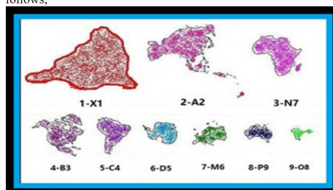
Figure 2: The ancient plates group led by ancient Jiazhou plate in the jigsaw recovery of the unique supercontinent 66 Ma ago.
