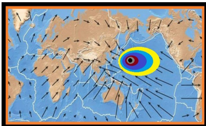
Figure 3: The HBH (Hint Black Hole) hinted by the motive trend of lithosphere globally.
